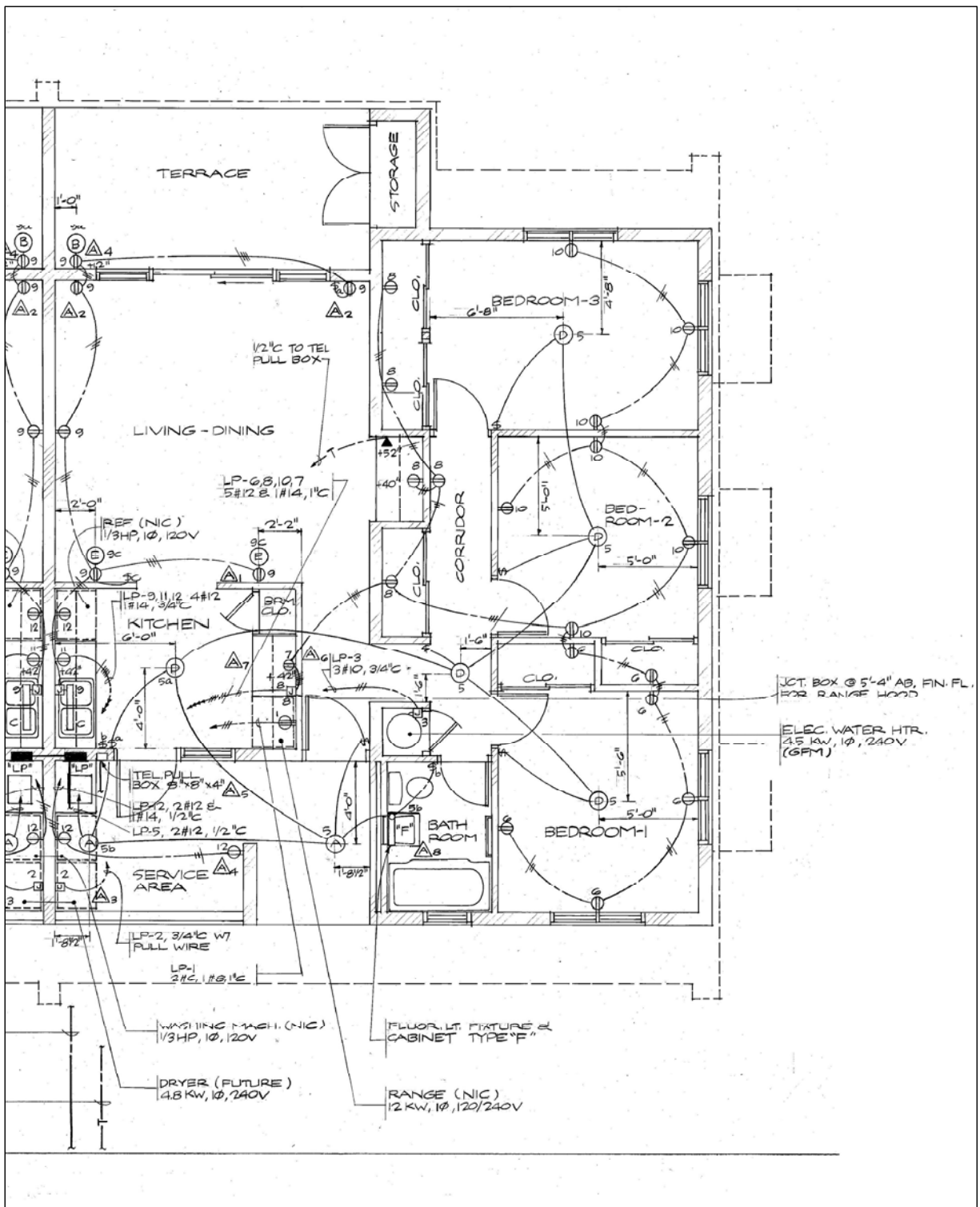
ELECTRICAL PLAN AS-BUILT (SIMILAR)
