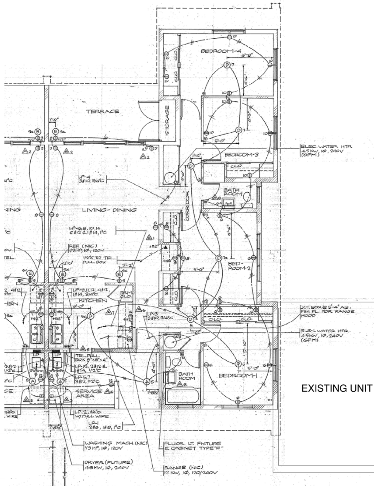
EXISTING ELECTRICAL 4-BEDRROOM FLOOR PLAN AS-BUILT
