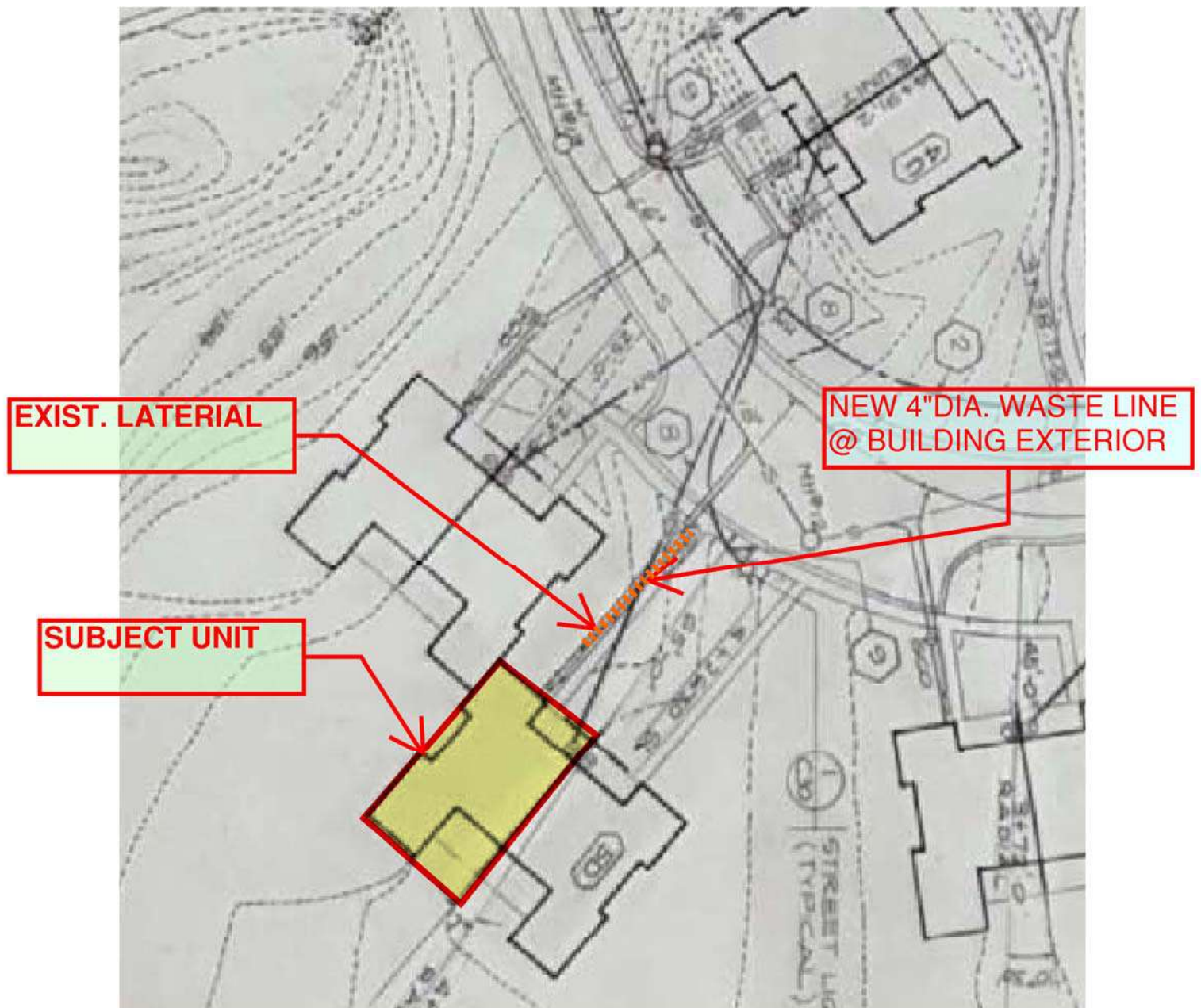
11B CALLE DAMIAN EXISTING SITE UTILITY PLAN
