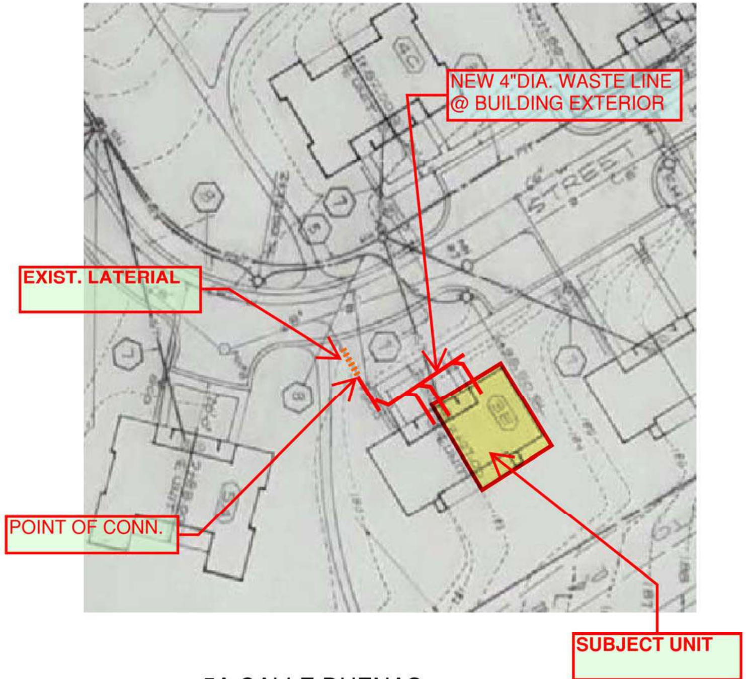
5A CALLE DUENAS EXISTING SITE UTILITY PLAN
