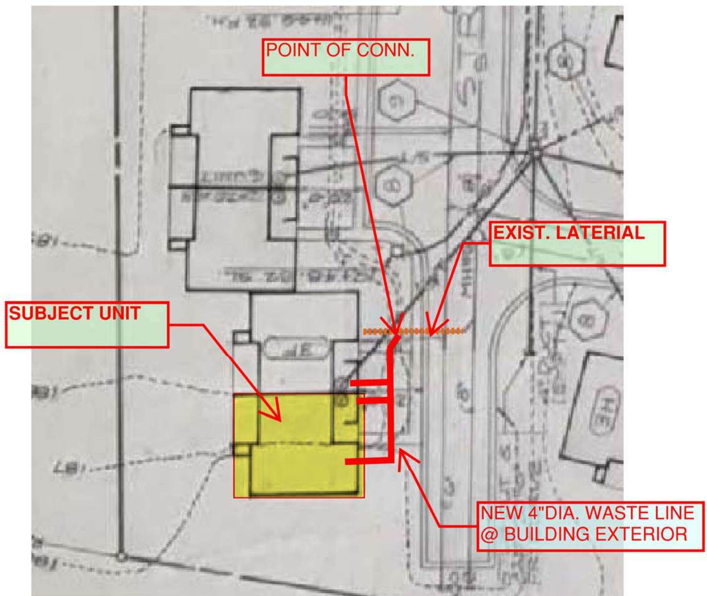
32B PAQUITO EXISTING SITE UTILITY PLAN
