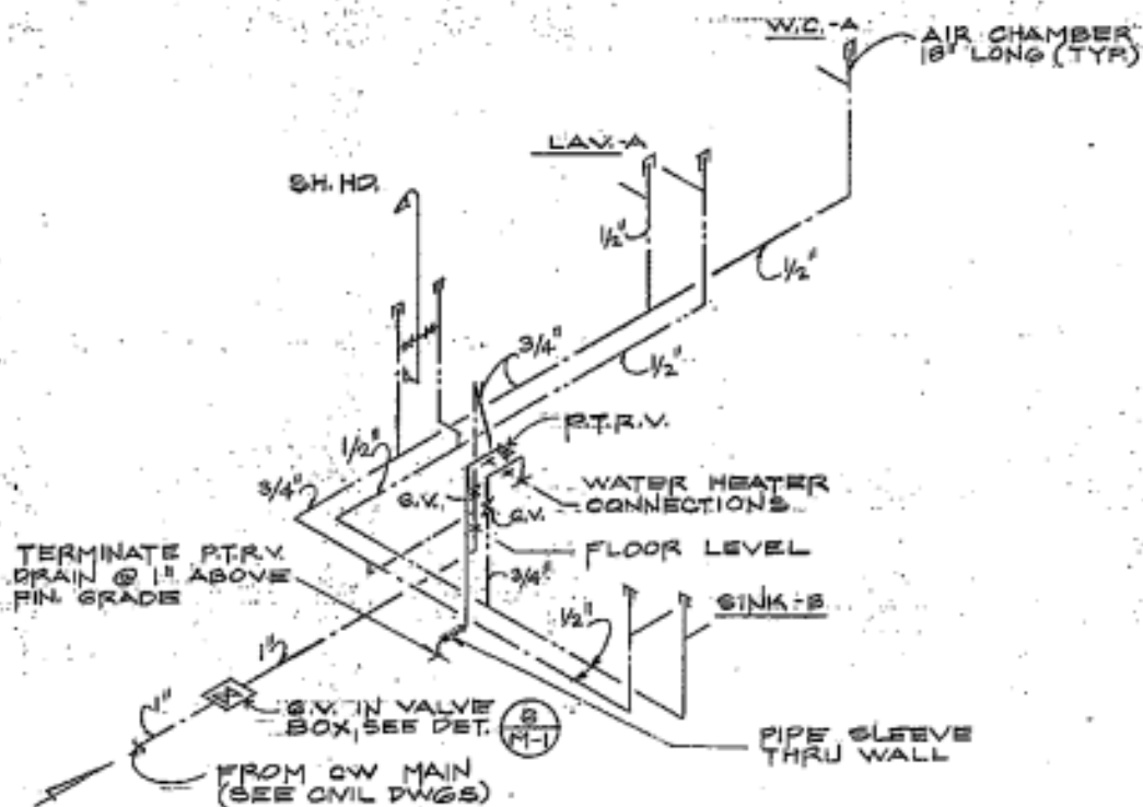
4 HW & CW ISOMETRIC DIAGRAM M-2 SCALE: NONE
