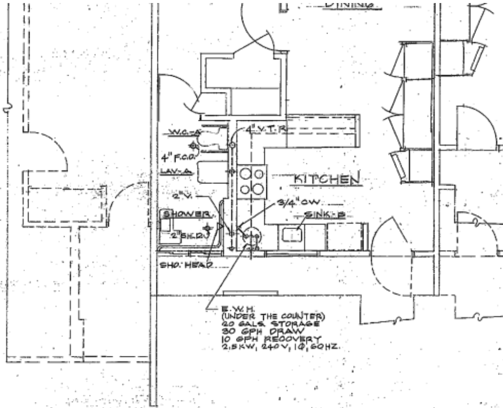
① ABOVEGROUND PIPING PLAN M-2 SCALE: 1/4" = 1'-0"
