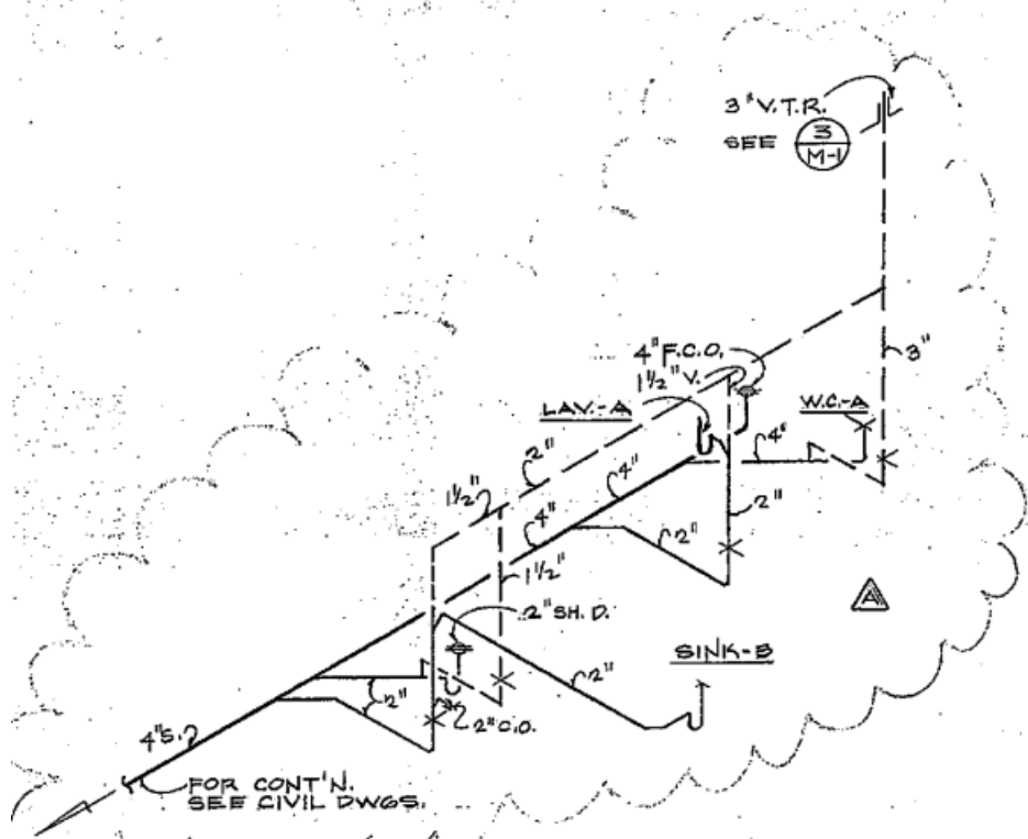
③ S, W, & V ISOMETRIC DIAGRAM M-2 SCALE: NONE
