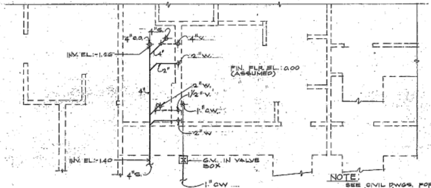
2 UNDERGROUND PIPING PLAN M-2 SCALE: 1/4" = 1'-0"
