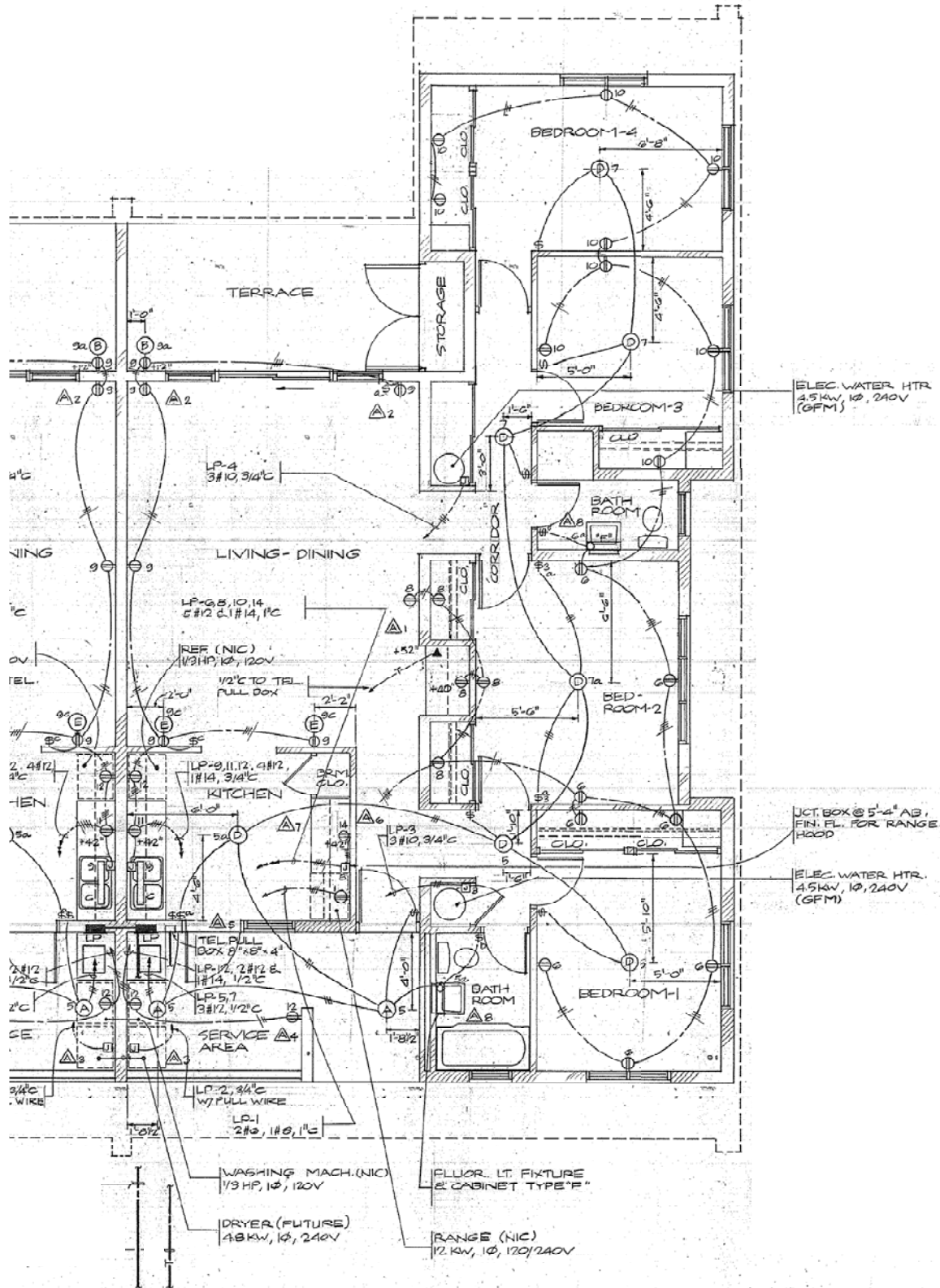
EXISTING ELECTRICAL 4-BEDRROOM FLOOR PLAN AS-BUILT
