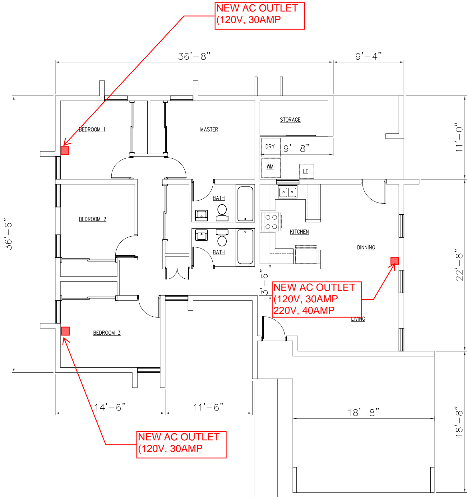
GH-35, 4-BEDROOM FLOOR PLAN
